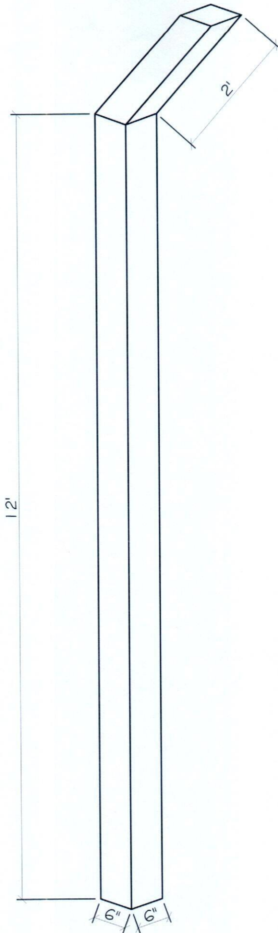
6" x6" 14'-0" fencing concrete post
